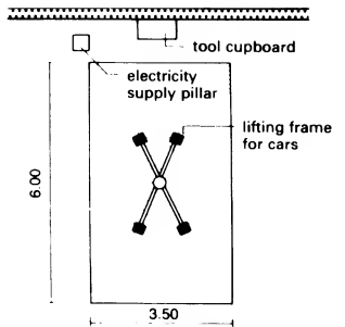
① Standard work area with lifting frame for cars 3.5m x 6.0m: hoist height 1.0m
